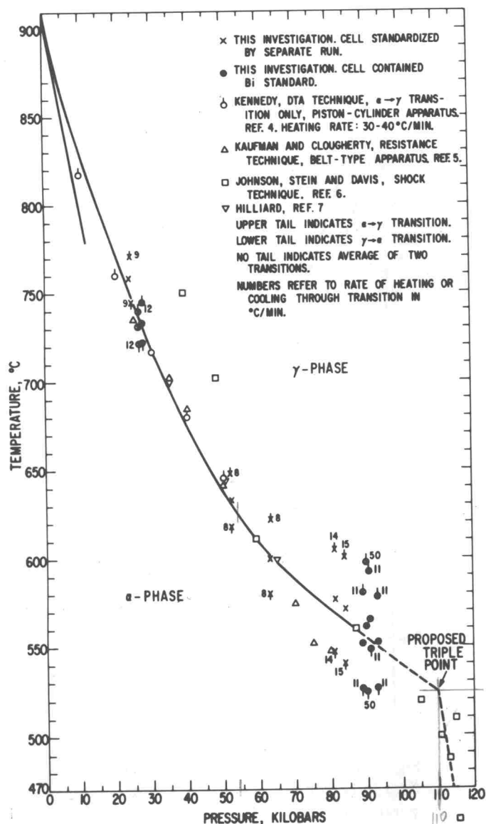
Fig. 4 Pressure-temperature curve for \alpha - \gamma transformation in iron
