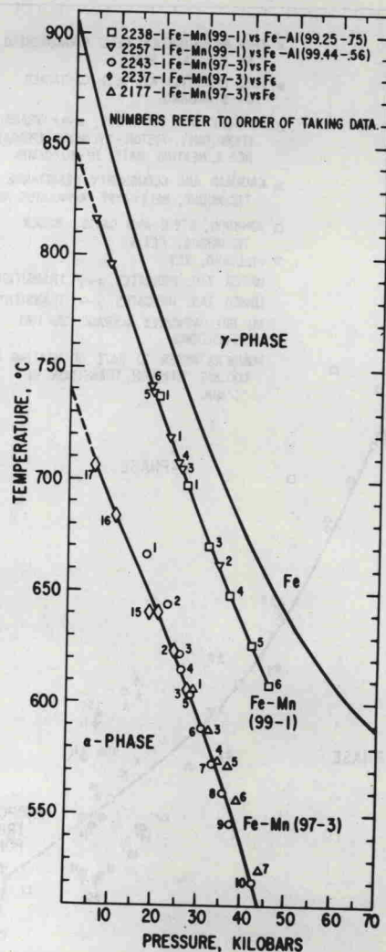
Fig. 6 P-T plots for \alpha - \gamma transformations in Fe-Mn alloys. Average temperature curves
