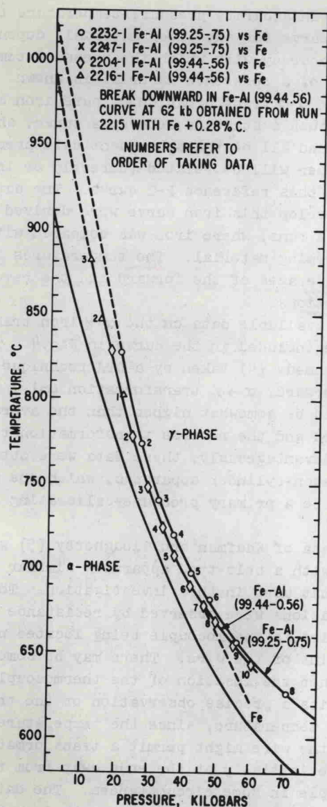
Fig. 5 P-T plots for \alpha - \gamma transformations in Fe-Al alloys. Average temperature curves
